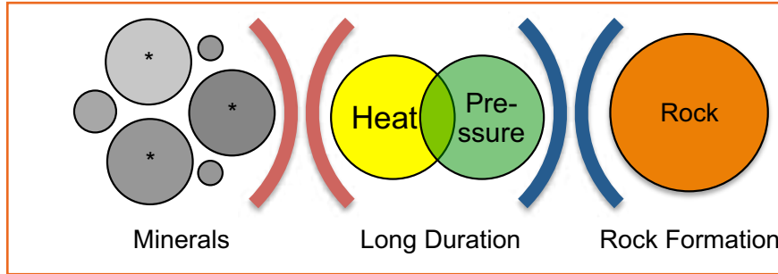
Fig. 1.2.2 Formation of rocks
